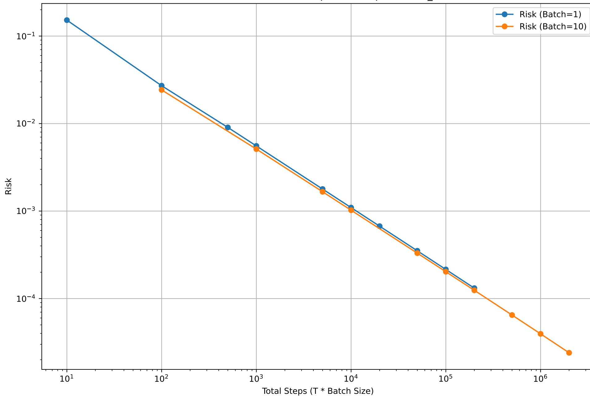
Slock Risk for Different Batch Sizes; \alpha=1.8 . optiized eta_star for each T
